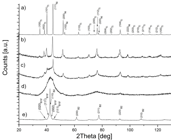
Fig. 3 X-ray diffraction patterns of powders at various stages of: mixed for 48 hrs (a); high-energy milling: 20 hrs (b), 60 hrs (c), 100 hrs (d) and after crystallization at 600°C (e)
