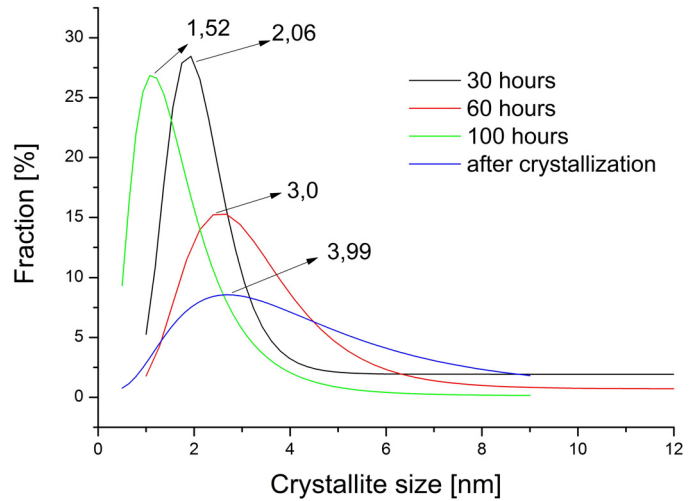
Fig. 7. Comparison of fitted lognormal function determined from histograms for the BCC phase after various milling times and crystallization
