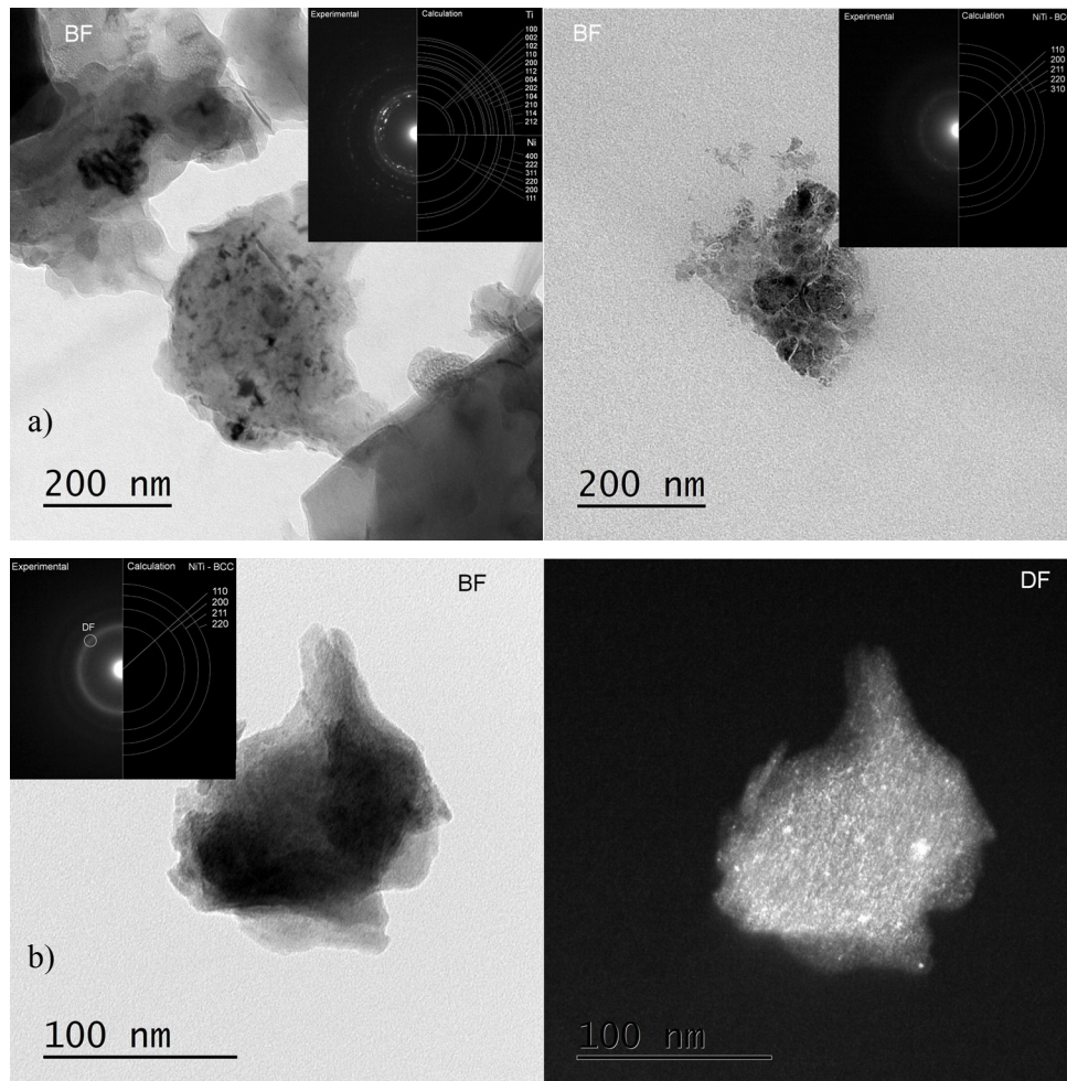
Fig. 4. TEM images (bright field – BF and dark field – DF) as well as SAED patterns observed for the powders milled after 20 hrs (a) and 100 hrs (b)
