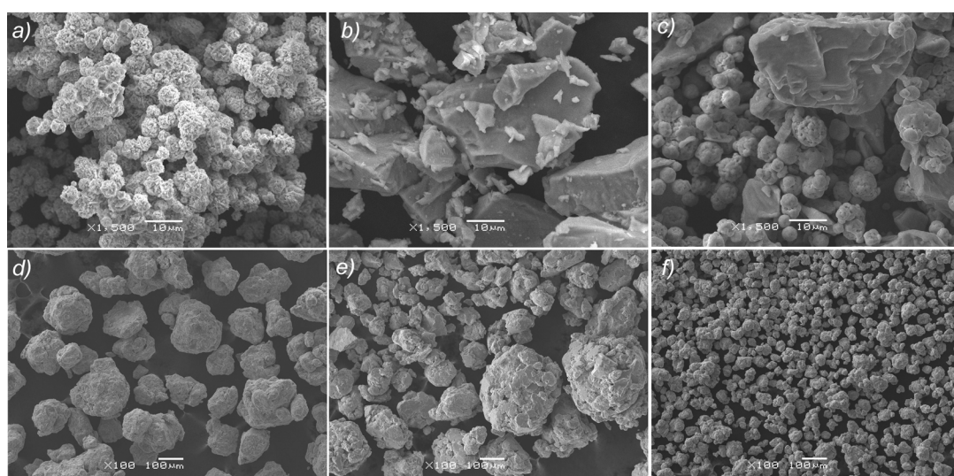
Fig. 1. SEM images observed for powders: a) nickel, b) titanium, c) mixture after 48 hours of homogenization, and after high energy ball milling d) 20 hrs, e) 60 hrs, f) 100 hrs
