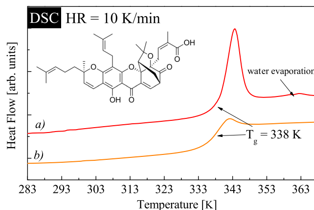
FIG. 2. DSC thermograms for the (a) as-obtained gambogic acid and (b) gambogic acid annealed at 373 \text{ K} for 3 \text{ min} prior to measurement. The inset presents the chemical structure of the investigated material.
