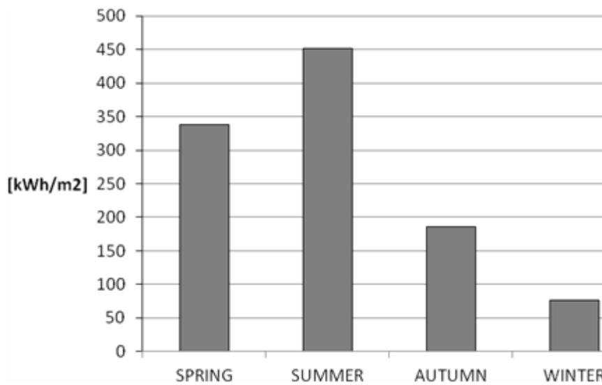
Fig.5. Average seasonal totals of irradiation on flat surface in Sosnowiec (2003 – 2013)
