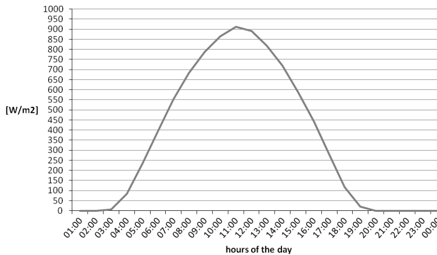
Fig.1. Daily course of global solar radiation in Sosnowiec (an example for cloudless day 17 June 2010)
