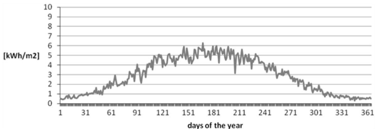
Fig.3. Annual course of daily averages radiation energy totals in Sosnowiec (2003 – 2013)
