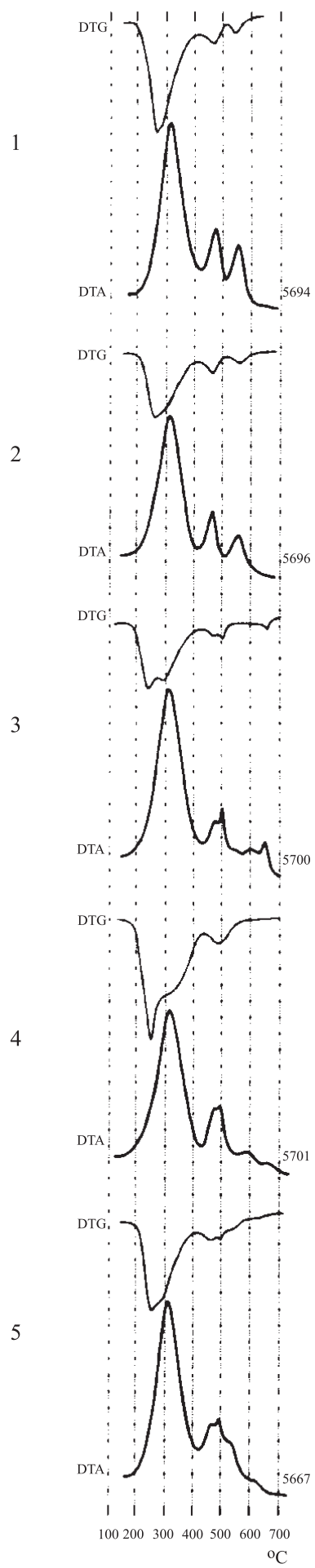
Fig. 5. DTA and DTG curves of Fucus vesiculosus with morphological differentiation: 1 – external part of thallus; 2 – bladder wall; 3 – internal part of thallus; 4 – core; 5 – whole thallus
