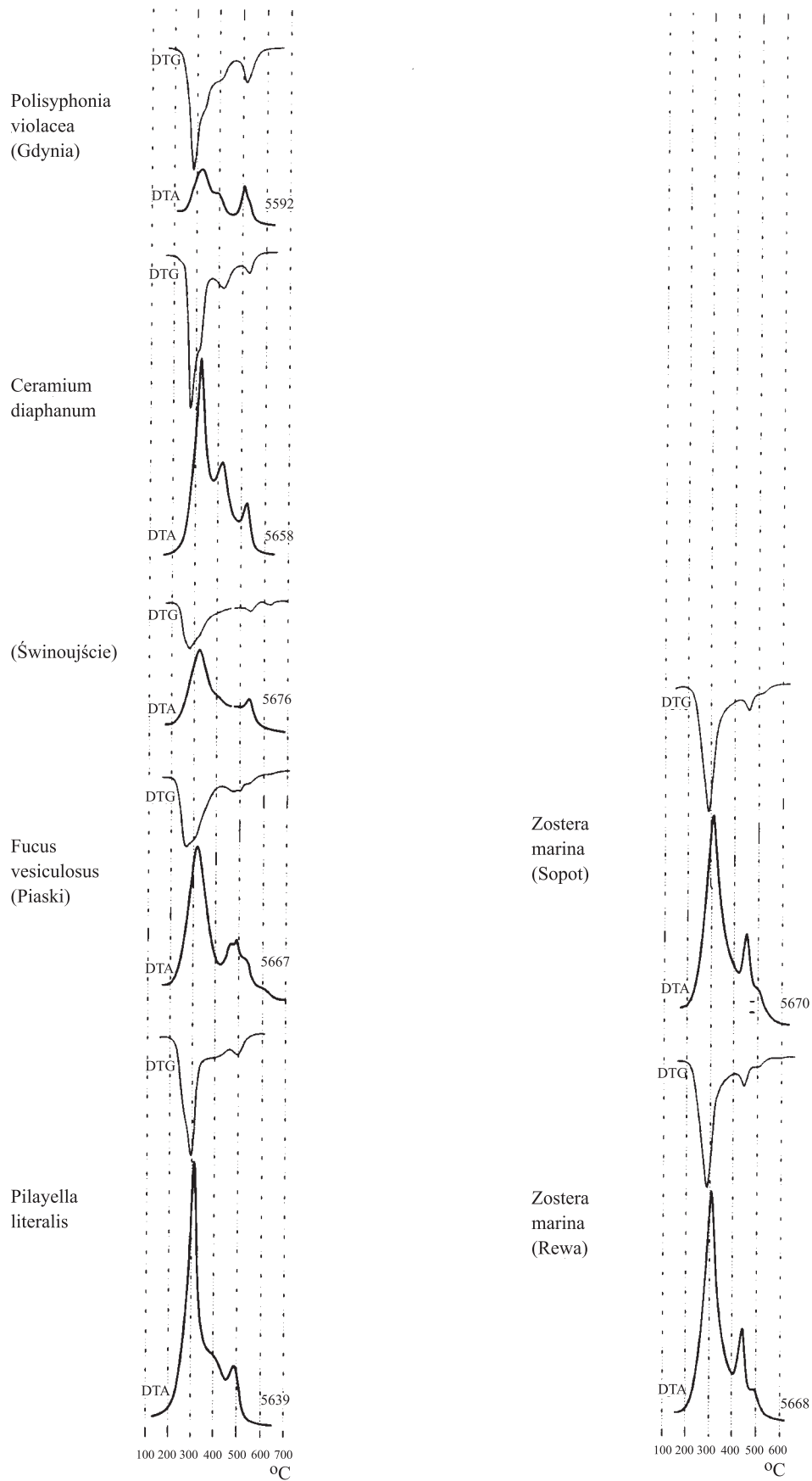
Fig. 4. DTA and DTG curves of different species of Rhodophyta and Phaeophyta, and Zostera marina from selected stations (name in parentheses)
