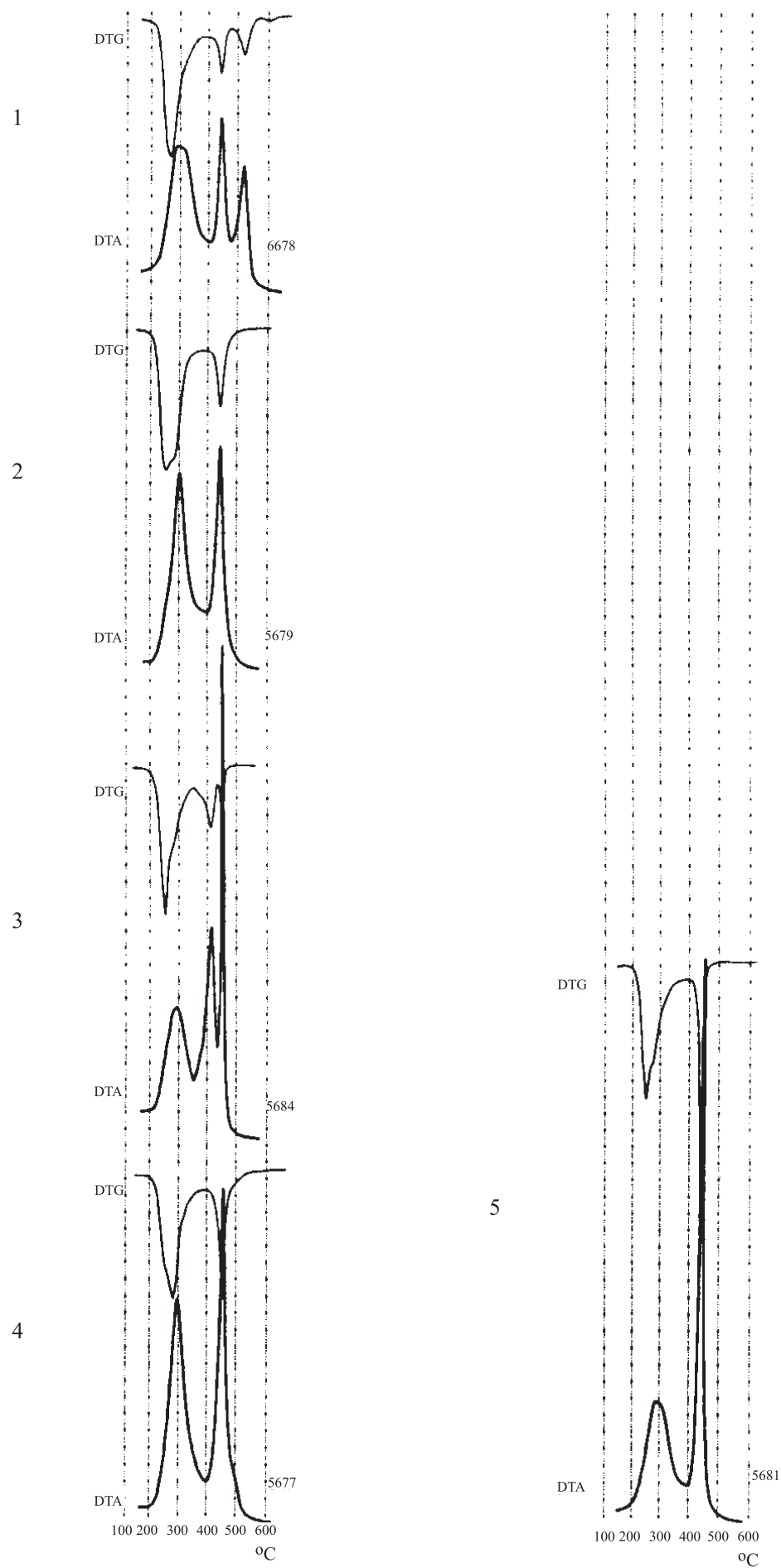
Fig. 6. DTA and DTG curves of Laminaria spp. from Spitsbergen with morphological differentiation: 1 – thin part (white) of thallus; 2 – thick part (brown) of thallus; 3 – core (brown part); 4 – rhizoidum; 5 – core (light-brown porous part)
