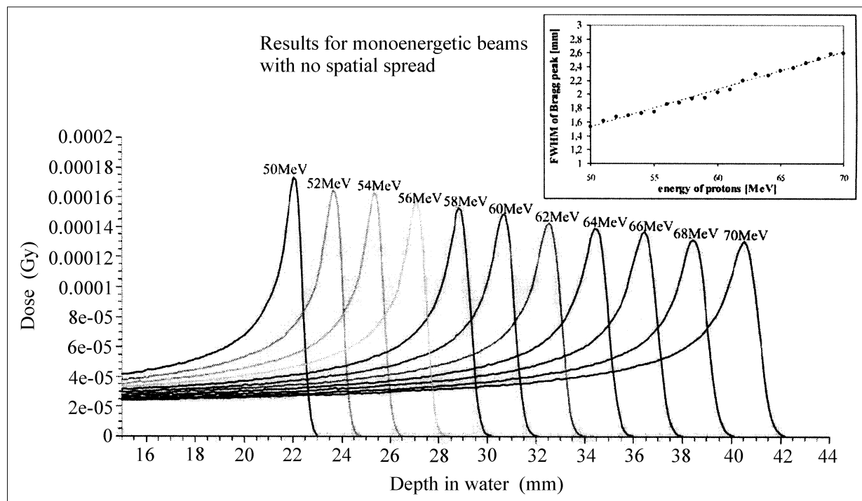
Fig. 1. Depth-dose characteristics of monoenergetic proton beams with no spatial spread; the dependence of energy of these beams on FWHM of the Bragg peak in the inset. Dose in Gy were determined in the bin volume for 10 000 protons.
