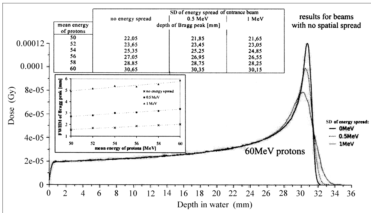
Fig. 2. Influence of the energy spread of the entrance beam on the depth-dose characteristics of 60 MeV protons; depth and FWHM of Bragg peak vs. mean energy of protons in the insets. Doses are determined as in Fig. 1.
