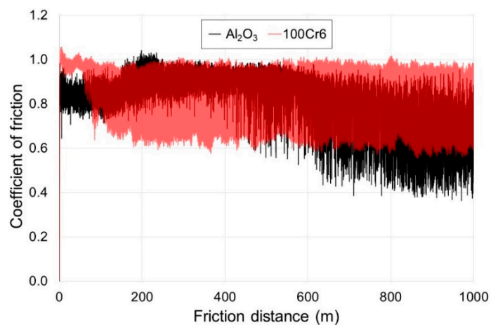
Figure 11. Diagram of the friction coefficient for titanium after annealing at 700 °C (72 h), recorded during friction with Al 2 O 3 and 100Cr6 balls.
