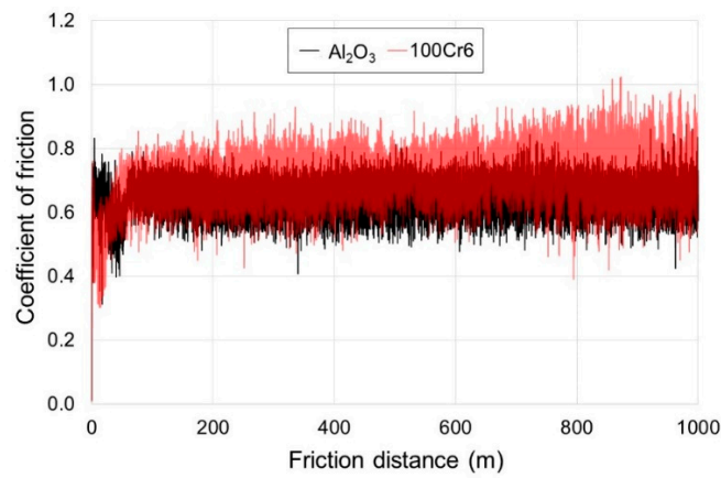
Figure 10. Diagram of the friction coefficient for non-oxidized titanium, recorded during tests with Al 2 O 3 and 100Cr6 balls.
