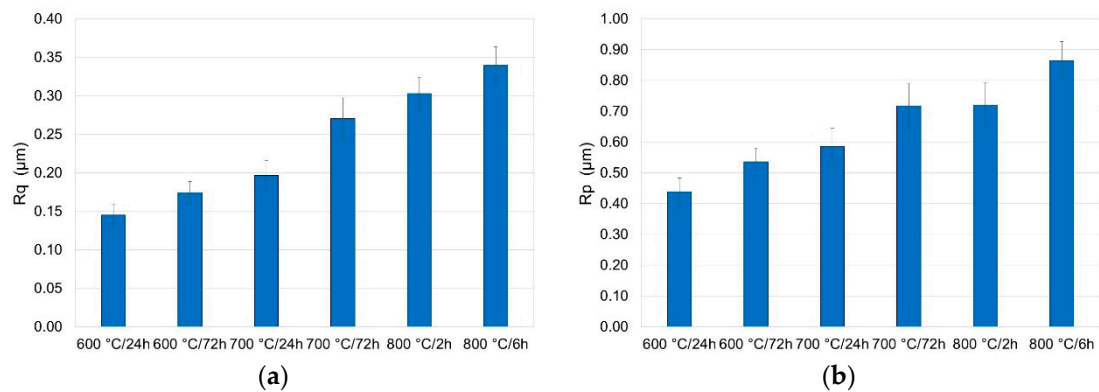
Figure 16. Surface roughness of titanium after annealing at 600, 700 and 800 °C (parameters (a) R_q , (b) R_p ).
