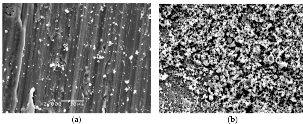
Figure 13. Microscopic photographs of the friction path formed on titanium after tests with 100Cr6 balls (corrugation wear: (a) light grey zone, (b) dark grey zone).
