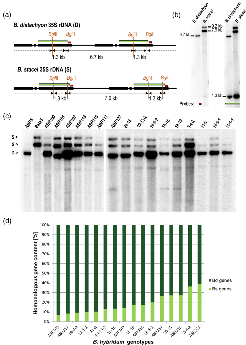
Figure 2. The structure of the 35S rDNA loci in Brachypodium hybridum . (a) The Bg/II restriction maps of the 35S rDNA units of Brachypodium distachyon and Brachypodium stacei . (b) Southern blot hybridization of the genomic DNA from B. distachyon and B. stacei that were subjected to digestion with Bg/II . The blot was hybridized with either the shorter (red rectangle, left panel) or longer (green rectangle, right panel) fragment of 25S rDNA. (c) Southern blot hybridization of the genomic DNA from B. distachyon , B. stacei and 16 B. hybridum genotypes that were subjected to digestion with Bg/II . The blot was hybridized with the short 25S rDNA probe. (d) Quantification of 35S rDNA homoeologues in different B. hybridum genotypes. The homoeologue gene number is denoted as a proportion of the D-genome or S-genome rDNA to the total rDNA.
