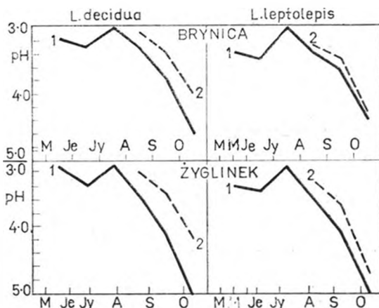
Fig. 2. Changes of pH in queous homogenates of the leaves on short shoots (1) and those on long ones (2) of L. decidua and L. leptolepis from Brynica and Żyglinek
