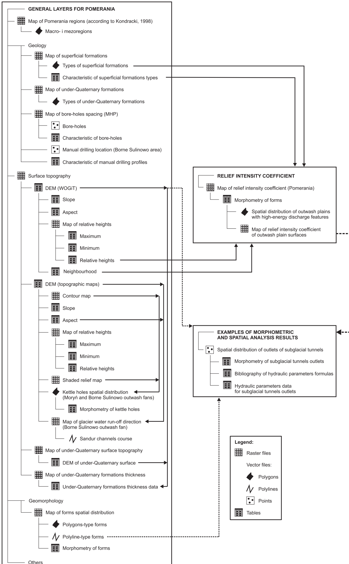
Fig. 4. Scheme of the Pomeranian relief intensity database
