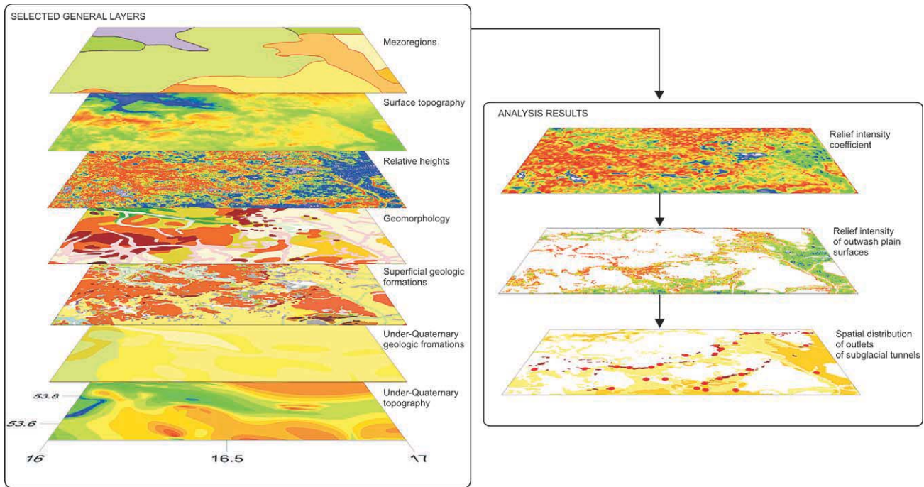
Fig. 3. Selected thematic layers used to develop and analyze the digital relief intensity map of Pomerania (fragment of the central part of the region in the vicinity of Szczecinek). Geographical coordinates are presented in the decimal degrees format
