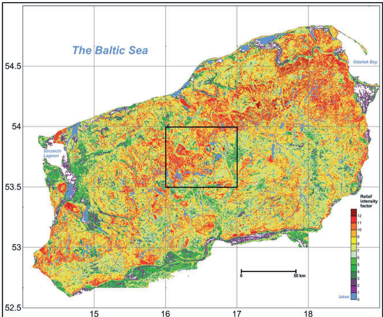
Fig. 2. Relief intensity map of Pomerania (worked out on the basis of the DEM from Wojskowy Ośrodek Geodezji i Teledetekcji and geological maps edited by Mojski, 1974–1981). Area in black box is presented on Fig. 3 as a visualization of exemplary thematic layers in geomorphological database. Geographical coordinates are presented in the decimal degrees format
