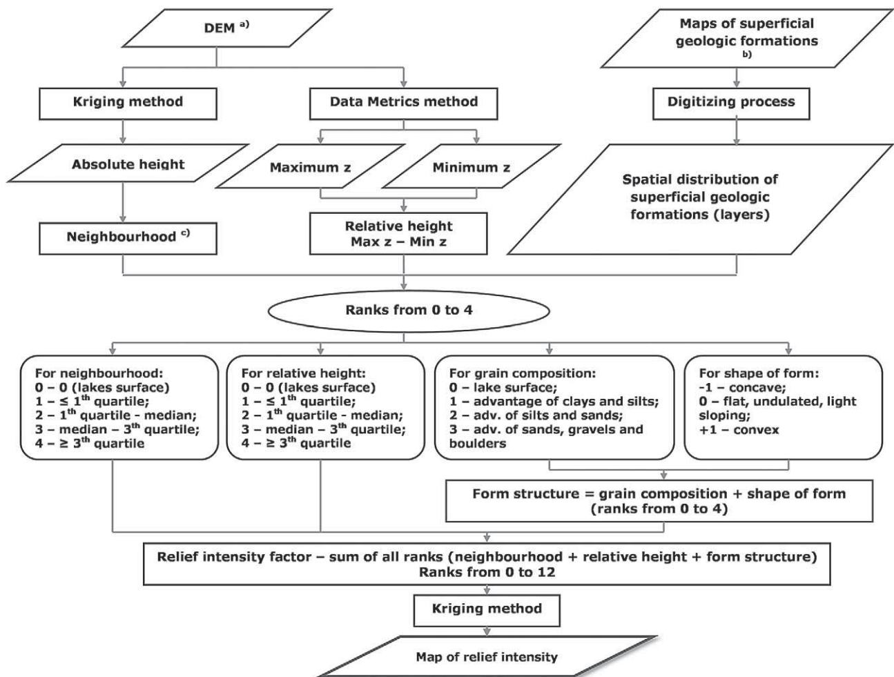
Fig. 1. Stages of the relief intensity coefficient calculations: a) DTED 2, Military Centre for Geodesy and Remote Sensing (for whole Pomerania); b) geological maps edited by Mojski (1974–1981), c) formula for one grid node; NH = [(AH_{(x_n,y_n)} - AH_{(x_{n+1},y_n)}) + (AH_{(x_n,y_n)} - AH_{(x_{n-1},y_n)}) + (AH_{(x_n,y_n)} - AH_{(x_n,y_{n+1})}) + (AH_{(x_n,y_n)} - AH_{(x_n,y_{n-1})})]^2 , where NH – neighbourhood, AH – absolute height, x, y – coordinates; the other operations apply to files
