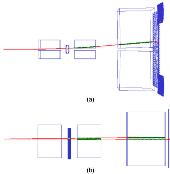
FIG. 4. Top (a) and side (b) view of the tracks of two high-energy particles going through the TPCs. The beam comes from the left. The track points are shown in green and the reconstructed TPC tracks are given in red. The two tracks are indistinguishable in the xz plane shown on plot (a). Plot (b), illustrating the yz plane, shows that only one of the particles is detected by the TOF-F wall on the right. This is marked by a big red dot. The other track is of an off-time particle that scattered elastically or quasielastically in the target and did not produce a signal in the TOF detector (busy processing the previous hit). The y position of the TOF-F hit is reconstructed based on the timing difference between the signals of the two PMTs at the ends of the hit scintillator bar.
