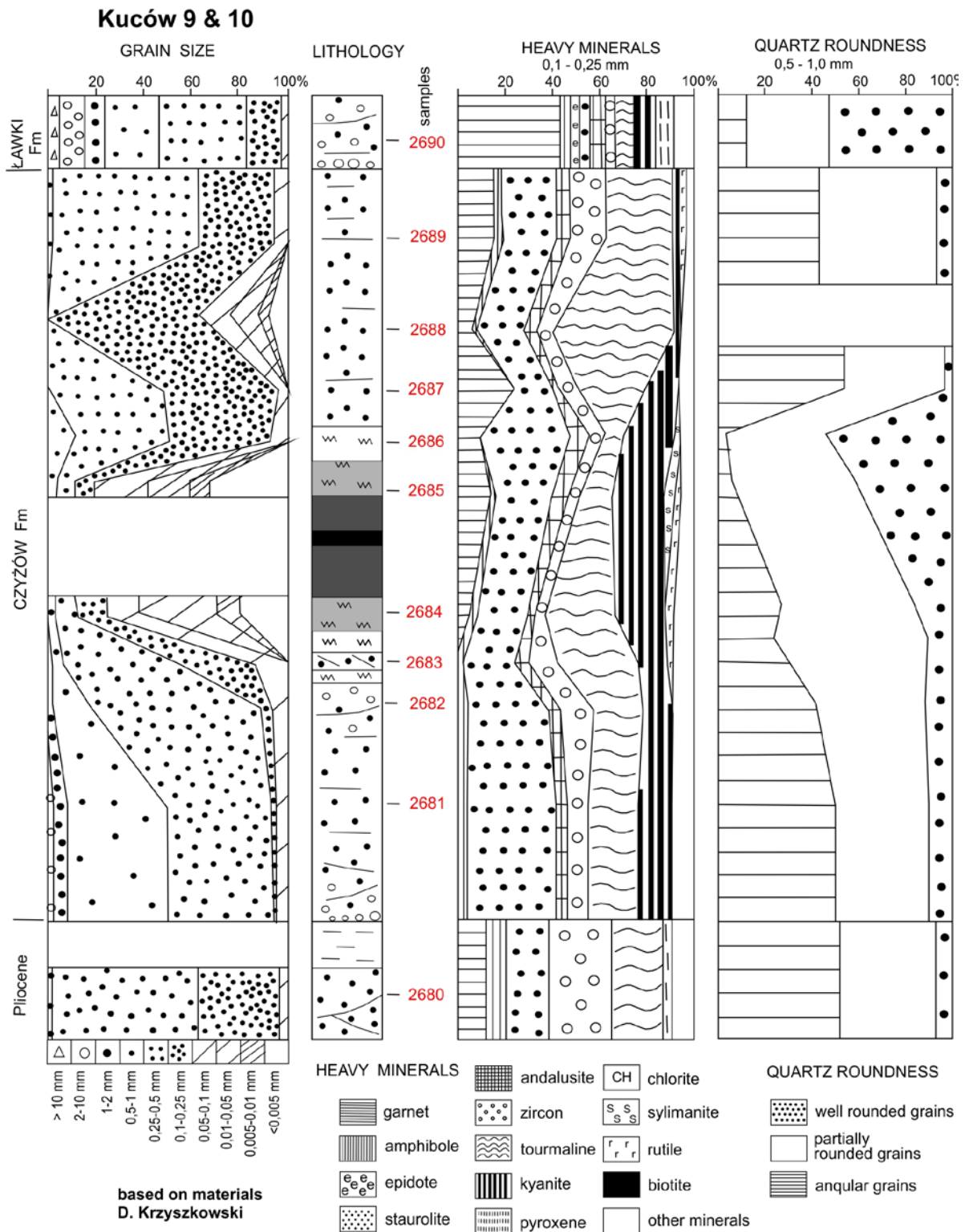
Fig. 8. Texture and petrography features of deposits in a central part of the Belchatów Field (sections Kuców 9 and 10).
