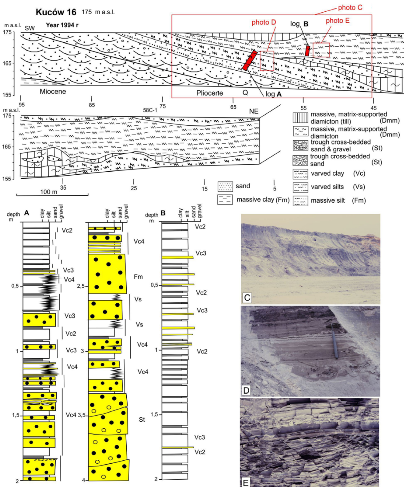
Fig. 3. Kuców 16 section: geology (top) and structure of deposits (bottom).
