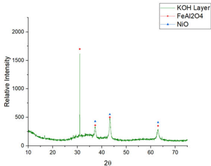
Figure 13. XRD obtained for the layer formed in OC4 alloy immersed in \text{KOH} .
