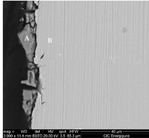
Figure 11. Cross-section image of OC4 alloy after 500 h in KOH at 380 °C, including EDX analysis at A-B point.
