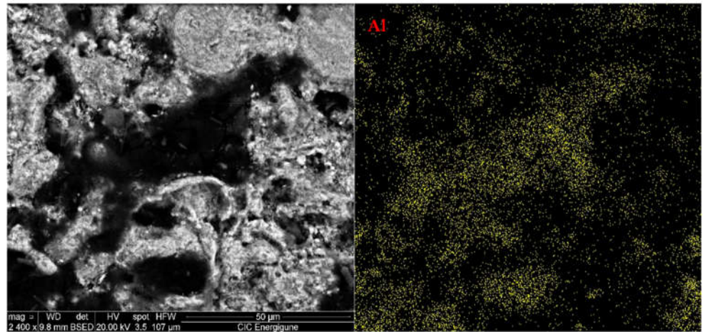
Figure 8. Superficial image magnification of OC4 alloy after 500 h in LiOH at 470 °C and mapping analysis (Al).
