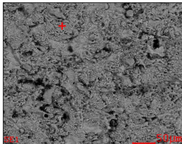
Figure 7. Superficial image of OC4 alloy after 500 h in LiOH at 470 °C.
