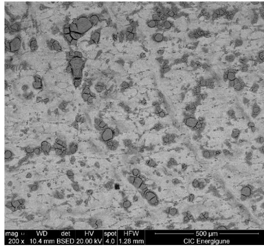
Figure 9. Superficial image of OC4 alloy after 500 h in KOH at 380 °C.
