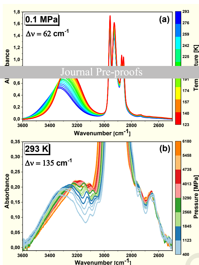
Figure 1. FTIR spectra of 2E1H measured at (a) T = 293 - 123 K and p = 0.1 MPa and b) T = 293 K and p = 400 - 6170 MPa in the frequency region of 3600 - 2500 \text{cm}^{-1} .
