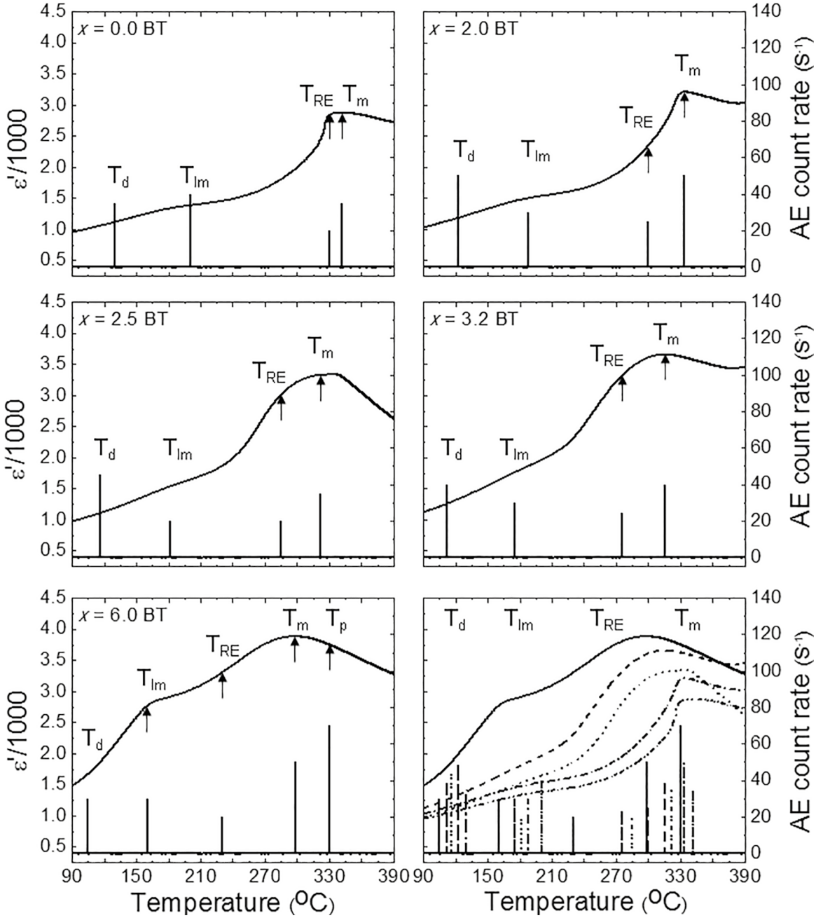
Figure 1. The plot of dielectric and acoustic emission data measured in Na_{0.5}Bi_{0.5}TiO_3-xBaTiO_3 relaxor ferroelectrics crystals (dash-dot-dot: x=0.00 ; dash-dot: x=0.02 ; dot: x=0.025 ; dash: x=0.0325 ; solid: x=0.06 ).
