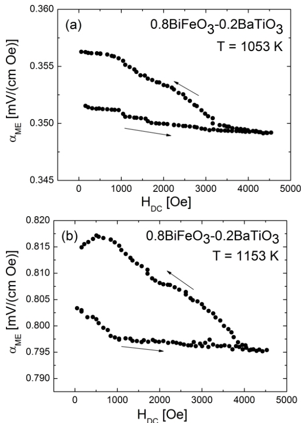
Fig. 4. Variation of \alpha_{ME} with H_{DC} for the samples with x = 0.8 , sintered under different technological conditions; (a) T = 1053 K (variant 1); (b) T = 1153 K (variant 3).
