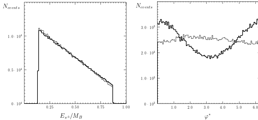
Fig. 3. As in the upper panels of figure 2 but for \delta_{\text{CP}} = 0.7 and a = 0.8 b .
