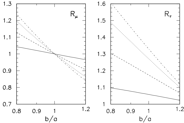
Fig. 1. The ratios R_\mu and R_\tau as functions of b/a for the phase \delta_{\text{CP}} = -\frac{1}{2}\arg(\lambda_{\text{L}}) = 0.1 (solid line), 0.3 (dashed), 0.5 (dotted) and 0.75 (dash-dotted). R_l(-\delta_{\text{CP}}) = R_l^{-1}(\delta_{\text{CP}}) .
