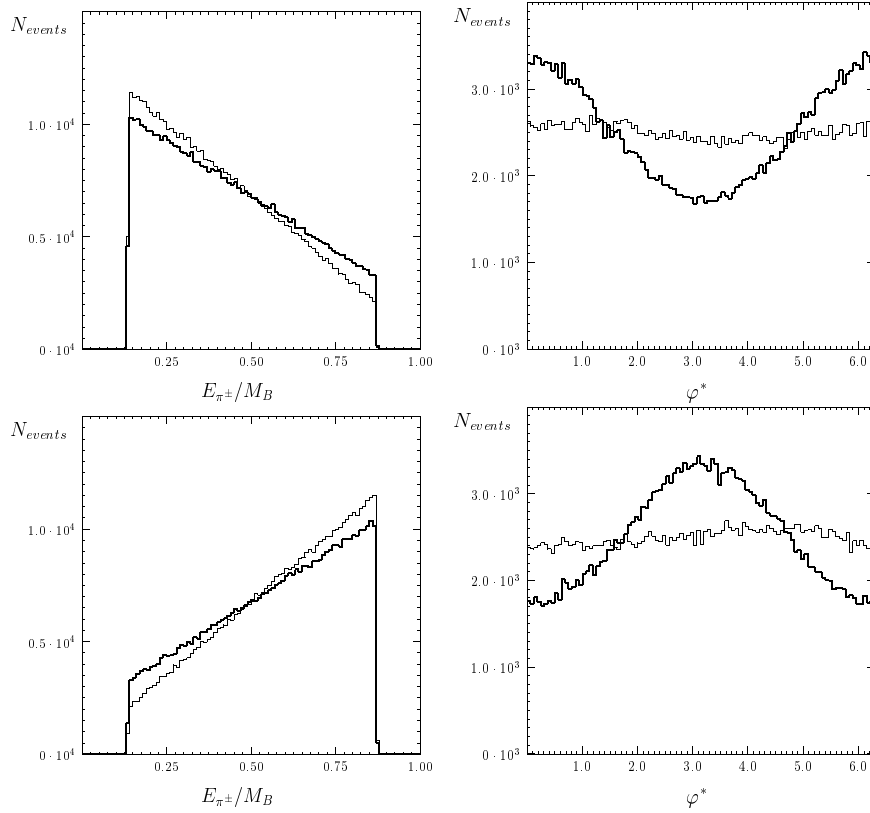
Fig. 2. Results for the CP violating phase \delta_{\text{CP}} = 0.7 and a = b . Left panels: Single \pi^\pm energy spectra in B^0(\bar{B}^0) \rightarrow \tau^+\tau^- , \tau^\pm \rightarrow \pi^\pm\nu_\tau(\bar{\nu}_\tau) . In the upper (lower) panel the thick line corresponds to the energy spectrum of \pi^- (of \pi^+ ) from B^0 decays and the thin line to the energy spectrum of \pi^+ (of \pi^- ) from \bar{B}^0 . Right panels: acoplanarity distributions of the \rho^+\rho^- decay products in B^0(\bar{B}^0) \rightarrow \tau^+\tau^- , \tau^\pm \rightarrow \rho^\pm\nu_\tau(\bar{\nu}_\tau) , \rho^\pm \rightarrow \pi^\pm\pi^0 . The thick lines correspond to the acoplanarity angle \varphi^* measured in B^0 decays and the thin ones are for the angle 2\pi - \varphi^* measured in \bar{B}^0 decays. Events in the upper (lower) panel have y_1y_2 > 0 ( y_1y_2 < 0 ).
