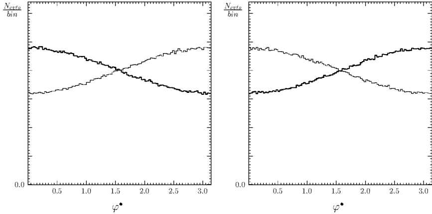
Fig. 6. The \rho^+\rho^- decay products' acoplanarity distribution angle, \varphi^\bullet , in the rest frame of the \rho^+\rho^- pair. A cut on the differences of the \pi^\pm\pi^0 energies defined in their respective replacement \tau^\pm rest frames to be of the same sign, selection y_1y_2 > 0 , is used in the left plot and the opposite sign, selection y_1y_2 < 0 , is used for the right plot. All smearing is included. Thick lines denote the case of the scalar Higgs boson and thin lines the pseudoscalar one.
