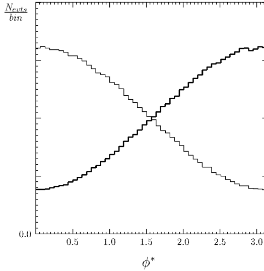
Fig. 1. The \pi^+\pi^- acoplanarity distribution (angle \phi^* ) in the Higgs boson rest frame. The thick line denotes the case of the scalar Higgs boson and thin line the pseudoscalar one.
