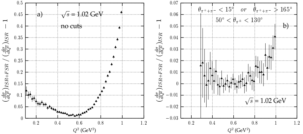
Fig. 3. Comparisons of ISR and FSR contributions to e^+e^- \rightarrow \pi^+\pi^-e^+e^- cross section at DAΦNE energy.
