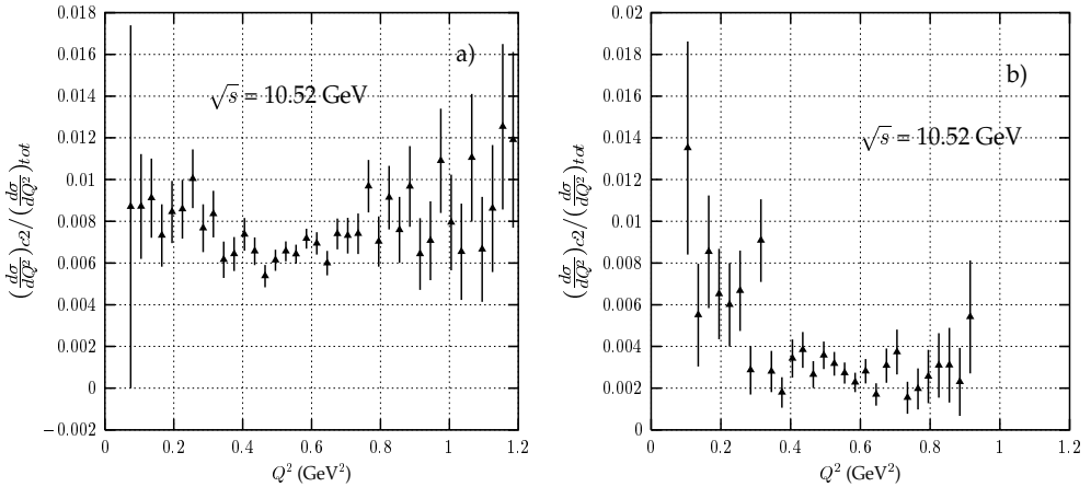
Fig. 7. Non-reducible pair production background at B-factory energy : (a) no cuts in (\frac{d\sigma}{dQ^2})_{tot} ; (b) for both (\frac{d\sigma}{dQ^2})_{c2} and (\frac{d\sigma}{dQ^2})_{tot} cuts on pion angles are imposed: 50^\circ < \theta_{\pi^\pm} < 130^\circ . For (a) and (b) c2 denotes additional cuts: (\theta_{e^+} < 20^\circ or \theta_{e^+} > 160^\circ) and (\theta_{e^-} < 20^\circ or \theta_{e^-} > 160^\circ) .
