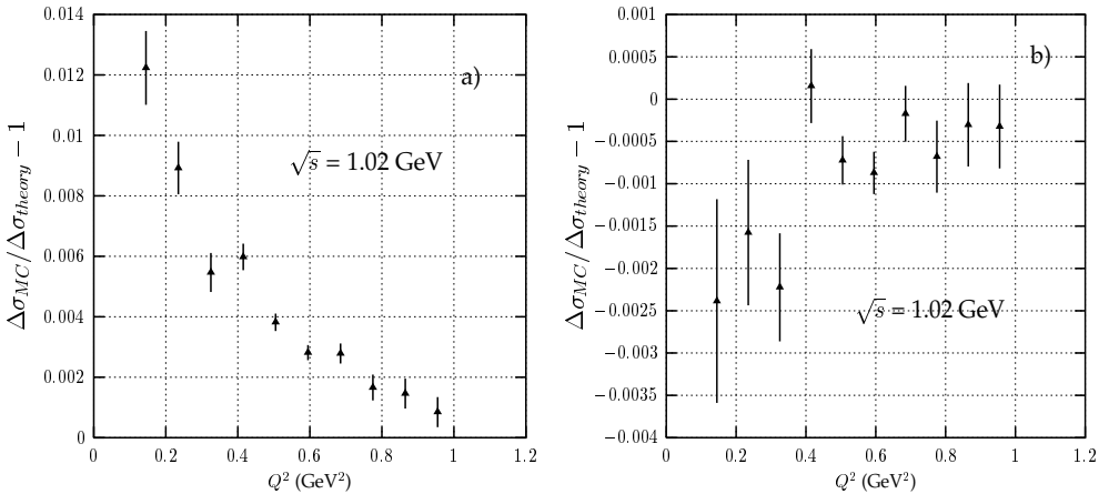
Fig. 2. EKHARA results compared with analytical results of [22] (see text for details). The errors come from MC integration.
