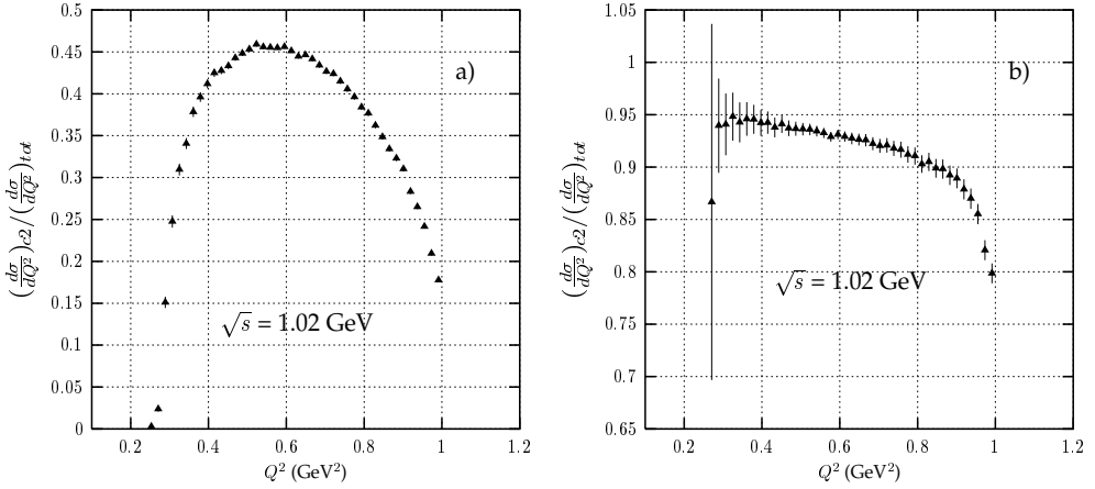
Fig. 6. Non-reducible pair production background at DAΦNE energy : (a) no cuts in (\frac{d\sigma}{dQ^2})_{tot} ; (b) for both (\frac{d\sigma}{dQ^2})_{c2} and (\frac{d\sigma}{dQ^2})_{tot} the following cuts are imposed: 50^\circ < \theta_{\pi^\pm} < 130^\circ , \theta_{\pi^+\pi^-} < 15^\circ or \theta_{\pi^+\pi^-} > 165^\circ and M_{tr} cut. For (a) and (b) c2 denotes additional cuts: (\theta_{e^+} < 20^\circ or \theta_{e^+} > 160^\circ) and (\theta_{e^-} < 20^\circ or \theta_{e^-} > 160^\circ) .
