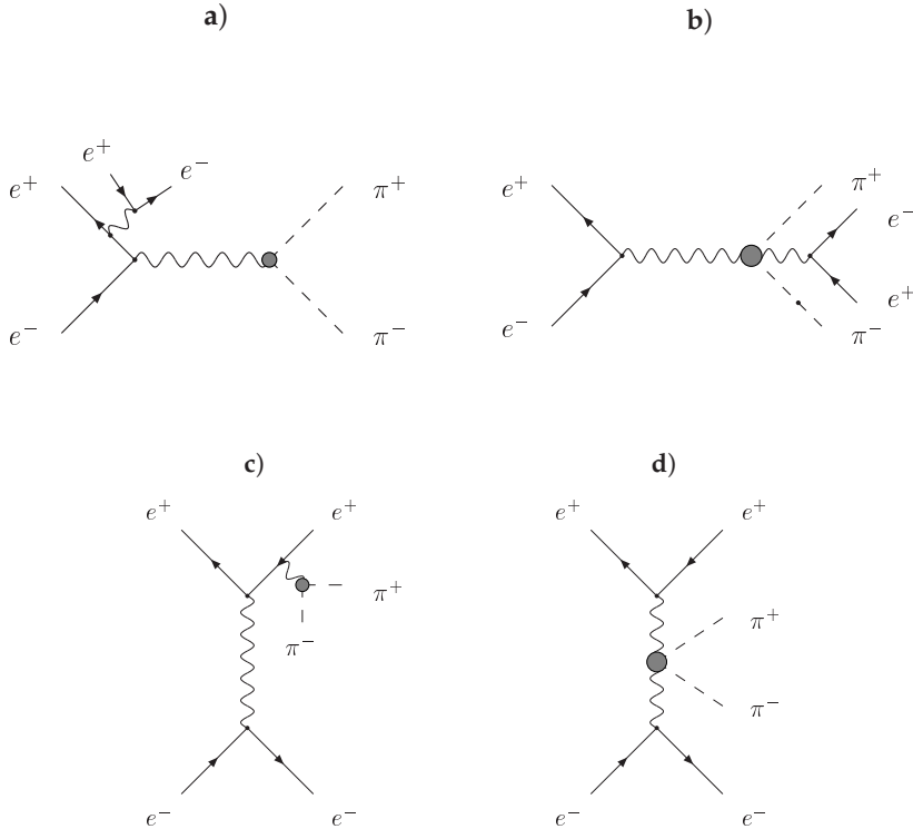
Fig. 1. Diagrams contributing to the process e^+(p_1)e^-(p_2) \rightarrow \pi^+(\pi_1)\pi^-(\pi_2)e^+(q_1)e^-(q_2) : initial state electron pair emission (a), final state electron pair emission (b), pion pair emission from t -channel Bhabha process (c) and \gamma^*\gamma^* pion pair production (d).
