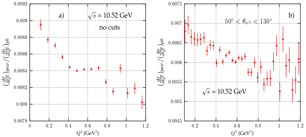
Fig. 5. Ratio of differential cross sections of the process e^+e^- \rightarrow \pi^+\pi^-e^+e^- (pair) and e^+e^- \rightarrow \pi^+\pi^- + \text{photon(s)} \text{ (ph)} .
