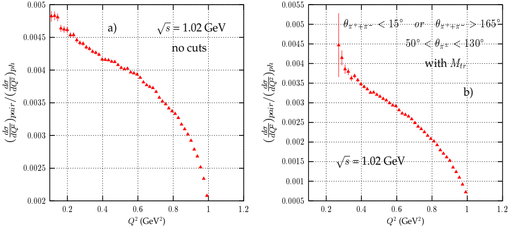
Fig. 4. Ratio of differential cross sections of the process e^+e^- \rightarrow \pi^+\pi^-e^+e^- (pair) and e^+e^- \rightarrow \pi^+\pi^- + \text{photon(s)} \text{ (ph)} .
